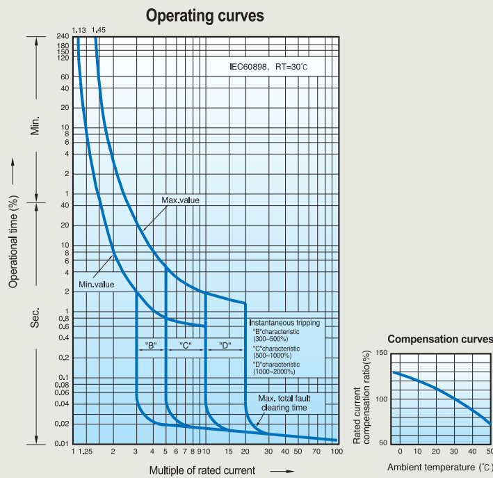
1.BKN, BKN-b, BKN-c, BKP, RKP, RKS, RKS-b (Temperature compensation table)(IEC60 898-1)
